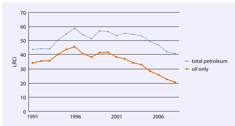
■ Fig. 4.7 Example of decline in EROI (Norwegian oil and gas; From [37])
