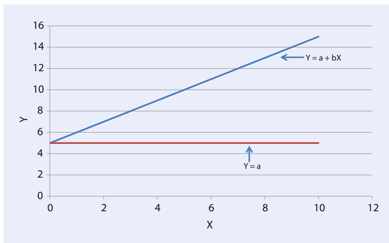
■ Fig. 16.1 Red Line: Linear with y = a constant (in this case 5) and Blue line: y = a constant plus a linear term of x
