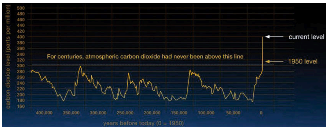
■ Fig. 23.6 Carbon emissions in historical perspective
